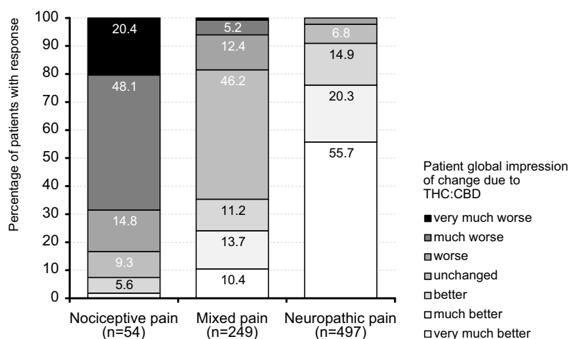
Figure 11 Patient global impression of change (PGIC) ratings for THC:CBD at end of the 12-week observation period. Abbreviations: THC, \Delta^9 -tetrahydrocannabinol; CBD, cannabidiol.
