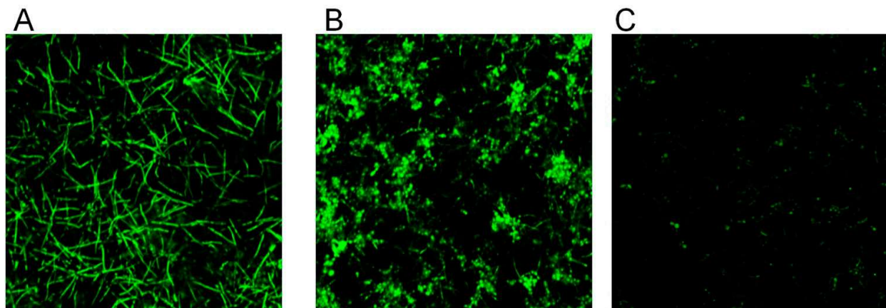
Figure 2. Effect of CBD on biofilm morphology. A–C. C. albicans –GFP biofilm were formed for 24 h in the absence of (A), presence of 25 µg/mL (B), or 100 µg/mL (C) CBD. The morphology of biofilms was visualized using NIKON confocal microscope with 488 nm laser excitation and collecting the data using the 535 nm green filter. Magnification 100×.
