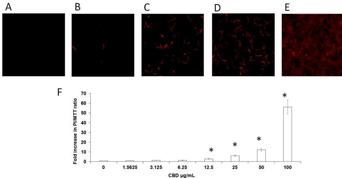
Figure 6. Membrane permeability of biofilm cells. C. albicans biofilms formed after a 24 h incubation with CBD were incubated with PI. A–E. PI-stained biofilms were observed by CLSM. PI staining of untreated control (A); biofilms treated with 3.12 µg/mL (B), 12.5 µg/mL (C), 50 µg/mL (D), or 100 µg/mL (E) CBD. Magnification 100×. (F). Relative PI fluorescence was measured in a plate reader. The ratios between dead cells and metabolically active cells in biofilms was calculated as PI fluorescence values divided on values obtained from MTT assay (PI/MTT ratio). Data are presented as a fold increase in PI/MTT ratio in treated biofilms compared to PI/MTT ratio in untreated biofilms. * Significantly lower than the untreated control ( p < 0.05 ).
