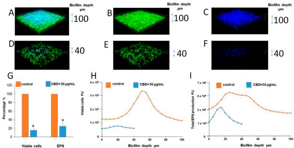
Figure 4. CLSM of biofilms. (A–F). CLSM 3D images of untreated and treated with CBD biofilms. (A,D). Merged images of metabolically active green fluorescence protein (GFP)-expressing (green color) fungal cells embedded in the extracellular polysaccharides (EPS) (blue color, ConA-stained); (B,E). Images of fungal cells alone (green color); C, F. Images of EPS alone (blue color); (A–C). Untreated control; (D–F). Biofilms were developed in the presence of 50 μg/mL CBD. Z-axis of 3D images indicates biofilm thickness. Magnification 100×. (G–I). Quantitative analysis of total EPS production and viable cells amount in each sample was calculated as blue and green fluorescence intensity, respectively, using Image J v3.91 software. Data are presented as total EPS production (I) and viable cells amount (H) in each layer of the biofilm (5 μm sections). Percentage of total EPS production and viable cells in biofilms treated with 50 μg/mL CBD is presented as area under the curve (AUC) and compared to untreated control (G). * Significantly lower than the untreated control ( p < 0.05 ).
