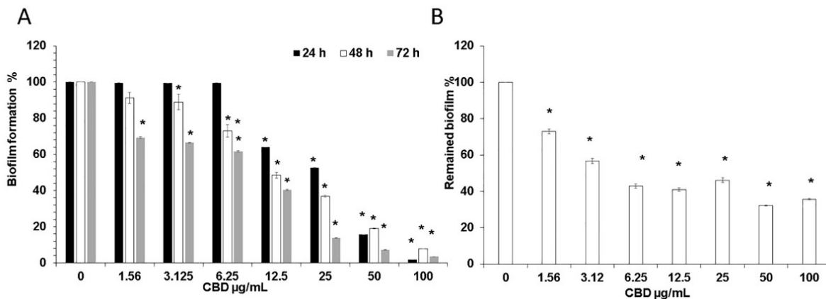
Figure 1. (A) Effect of CBD on C. albicans biofilm formation. C. albicans yeast cells were incubated with various concentrations of CBD for 24, 48, and 72 h at 37 °C; (B) Effect of CBD on preformed biofilms. Biofilms of C. albicans which were 24 h-old were exposed for 24 h to various concentrations of CBD and the metabolic activity of biofilm cells was measured using the MTT assay. The values of the untreated control were set to 100%. * Significantly lower than the untreated control ( p < 0.05 ).
