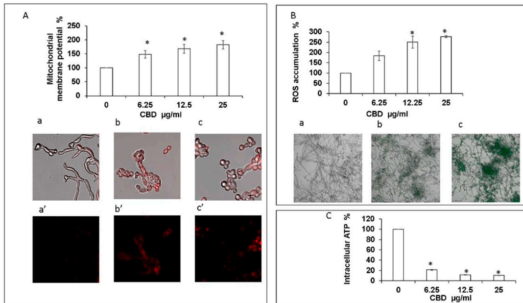
Figure 5. Assessment of mitochondrial function and ROS production. (A). Effect of CBD on C. albicans mitochondrial membrane potential (MMP) as determined by DiOC2(3). * Significantly higher than the untreated control ( p < 0.05 ); Mito Tracker Red-stained biofilms were observed by CLSM. Phase-contrast and Mito Tracker Red stain merged images (a–c), or Mito Tracker Red stain (a'–c') of untreated control (a,a'); biofilms treated with 12.5 \mu\text{g/mL} (b,b') or 25 \mu\text{g/mL} (c,c') of CBD. Magnification 600 \times . (B). Effect of CBD on ROS accumulation. C. albicans biofilms formed in the absence or presence of CBD were loaded with DCFHDA and the relative fluorescence intensities (RFI) of the biofilms were measured in a plate reader. The RFI values were normalized to the amount of metabolically active cells in biofilms assessed by MTT assay. * Significantly higher than the untreated control ( p < 0.05 ). Fluorescence images of untreated control (a), biofilm treated with 6.25 \mu\text{g/mL} (b) and 25 \mu\text{g/mL} (c) of CBD were captured by CLSM. Magnification 200 \times . (C). Effect of CBD on intracellular ATP levels. C. albicans biofilms formed in the absence or presence of CBD were analyzed for ATP content using the BacTiter-Glo reagent. * Significantly lower than the untreated control ( p < 0.05 ).
