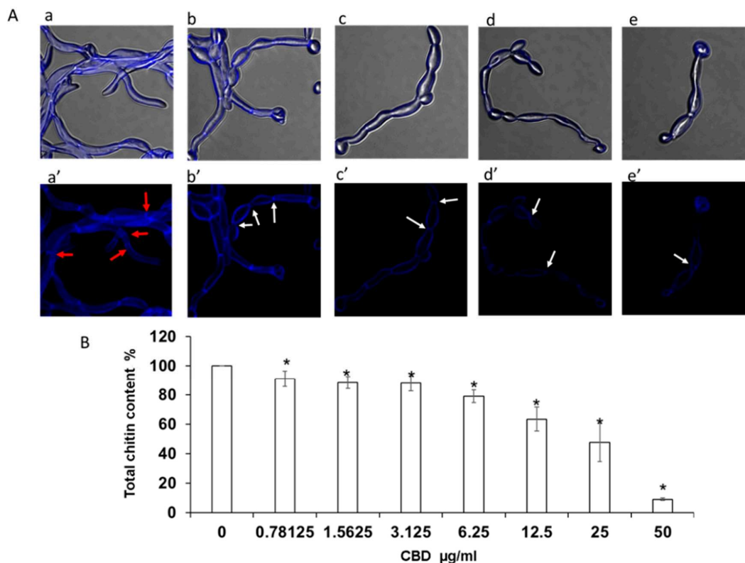
Figure 3. Determination of chitin content in biofilms. C. albicans biofilms after exposure to CBD for 24 h were stained with calcofluor white (CFW) for 5 min in the dark. (A). CFW-stained biofilms were observed by confocal laser scanning microscopy (CLSM). Phase-contrast and CFW stain merged images (a–e); CFW stain (a'–e') of untreated control (a,a'); biofilms treated with 6.25 \mu\text{g}/\text{mL} (b,b'), 12.5 \mu\text{g}/\text{mL} (c,c'), 25 \mu\text{g}/\text{mL} (d,d'), 50 \mu\text{g}/\text{mL} (e,e') of CBD. Red and white arrows indicate true septa and constrictions at the septal junctions, respectively. Magnification 600 \times . (B). Total chitin content was measured according to the CFW fluorescence intensity measured in a plate reader. Data are presented as percentage of the untreated control. * Significantly lower than the untreated control ( p < 0.05 ).
