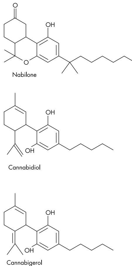
Figure 3 Chemical structure of nabilone, cannabidiol, and cannabigerol.
